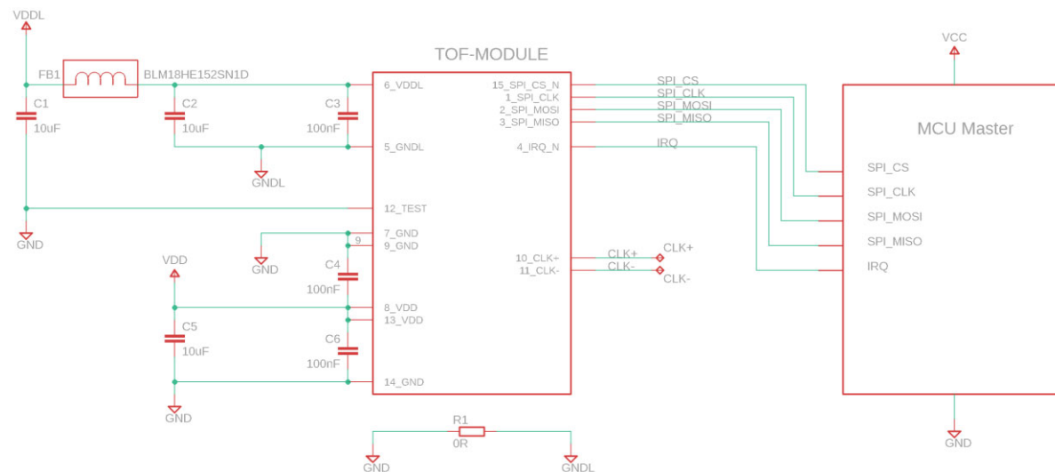
Figure 11: Application Schematic
