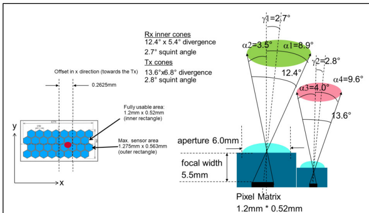
Figure 6: Field-of-View (FoV) Description of the Sensor
