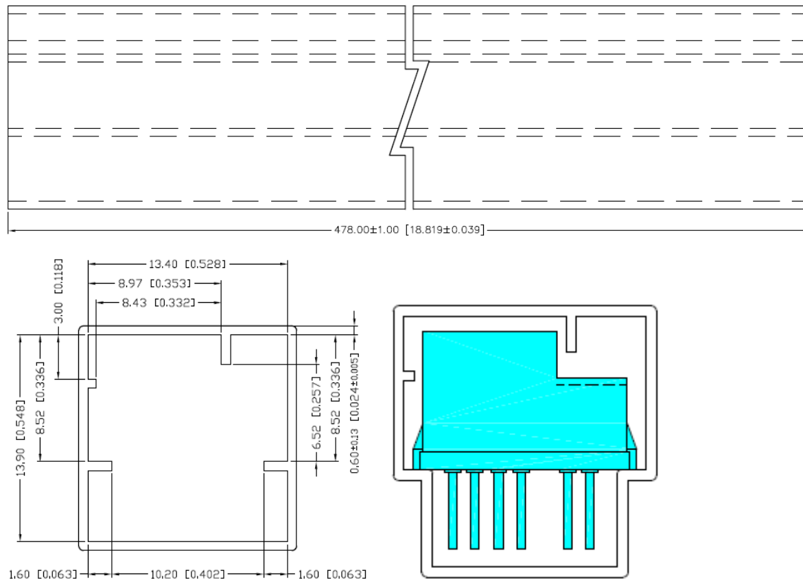
Figure 15: Packing Details
