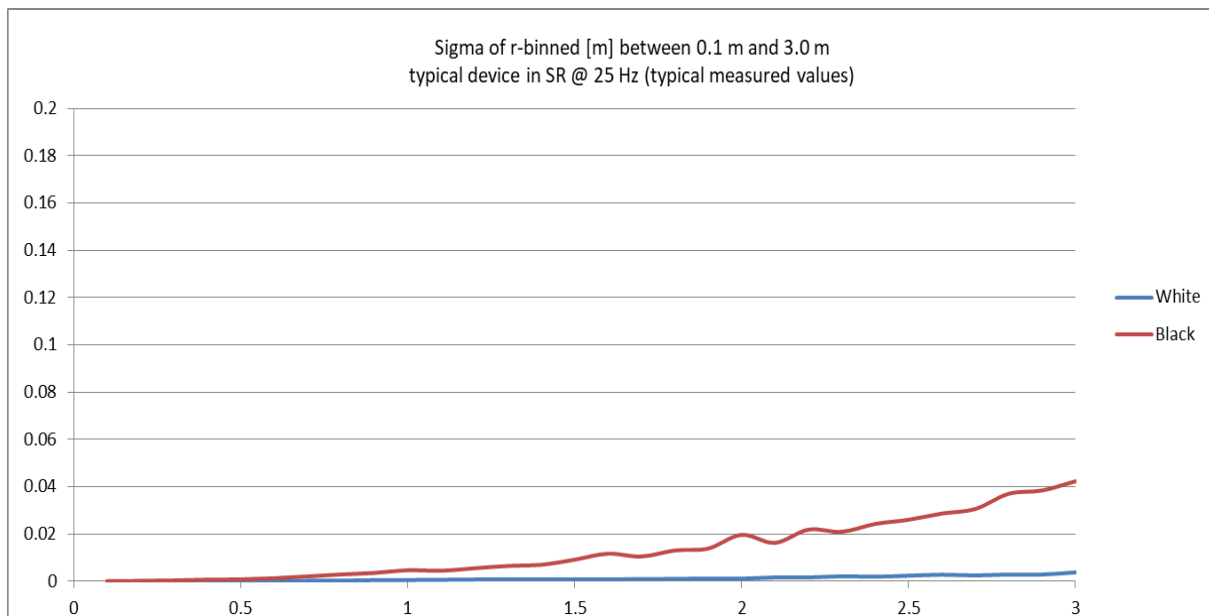
Figure 9: Standard Deviation Distance Measurement of All 32 Binned Pixel Values in Short Range Mode at a Frame Rate of 25 Hz, Laser Class 1 Lux and 1k Lux Ambient Light, Planar Targets
