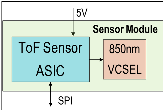
Figure 3: Block Diagram of AFBR-S50MV85I
