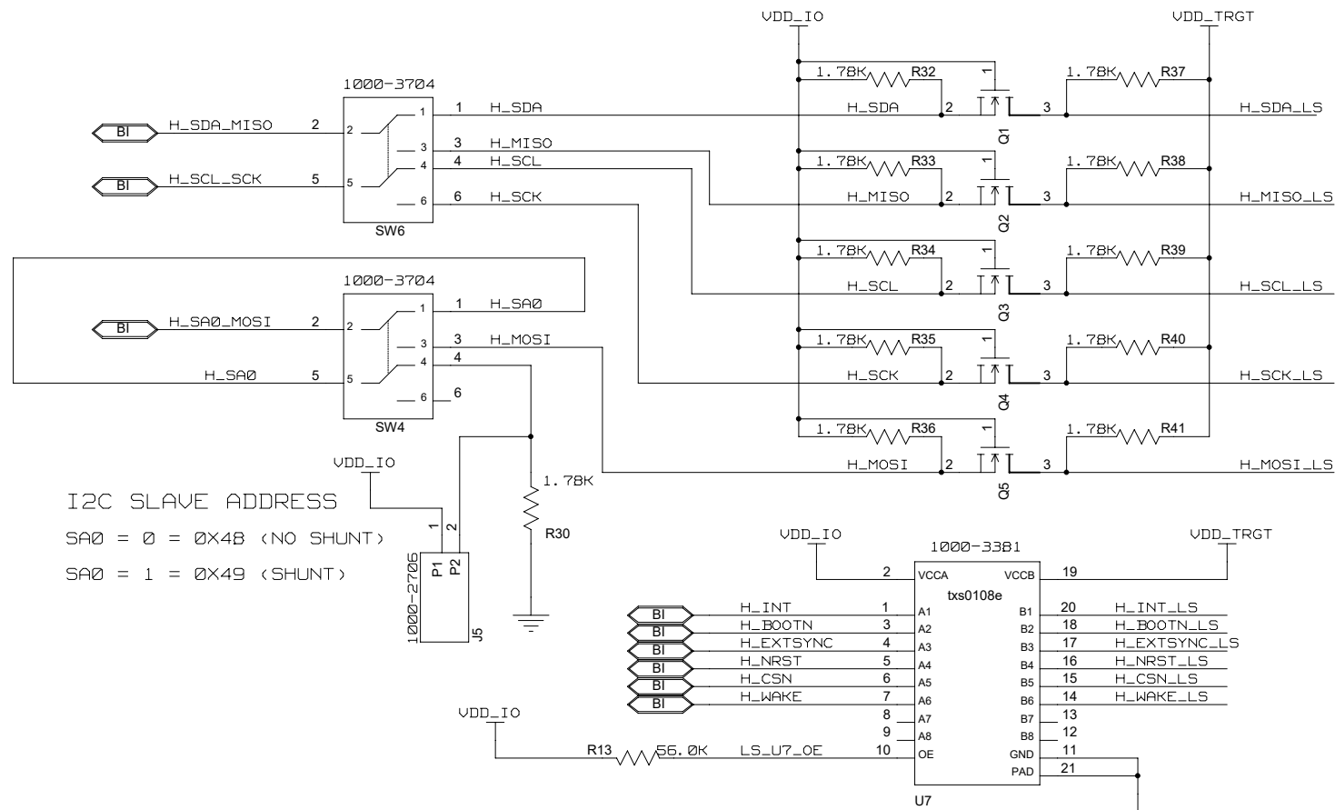
HOST LEVEL SHIFTING (FOR ARDUINO, NUCLEO, AND BEAGLEBONE)
