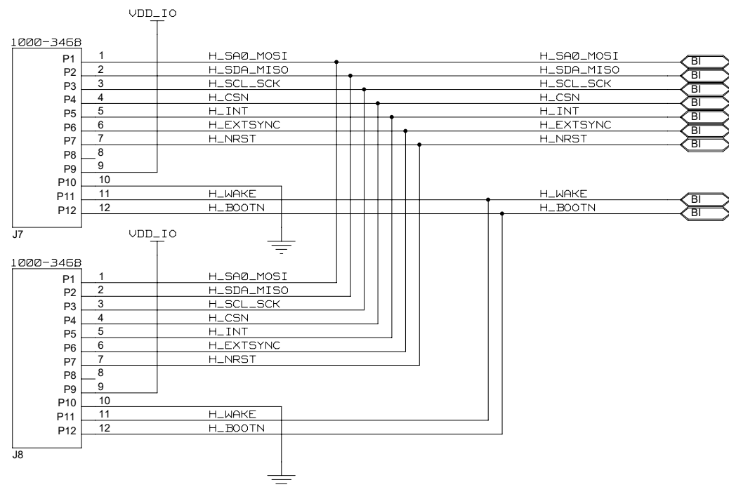
HOST INTERFACE (NO LEVEL SHIFTING)
