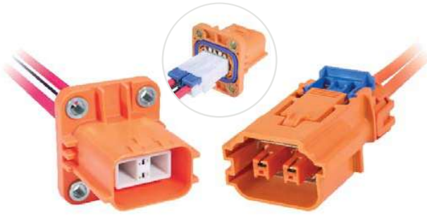
2 Way 180° Connection System with Pluggable Inner Connector
