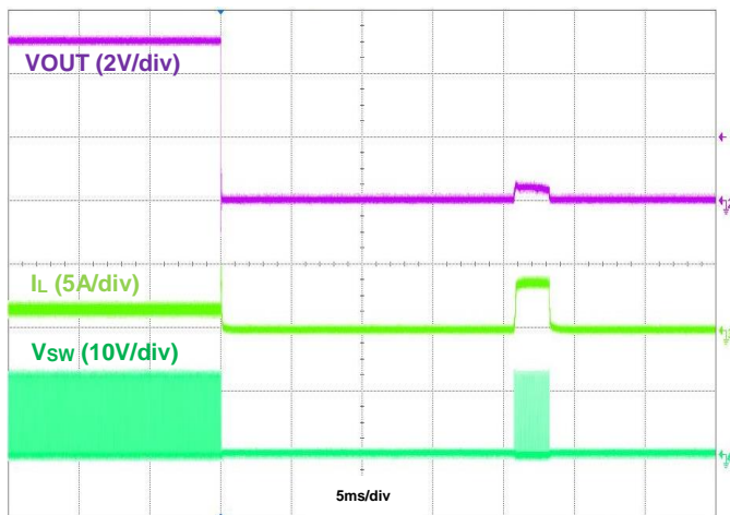
Figure 22. Output Short Protection, IOU = 1.5A
