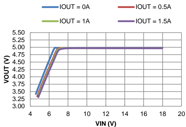
Figure 5. Line Regulation
