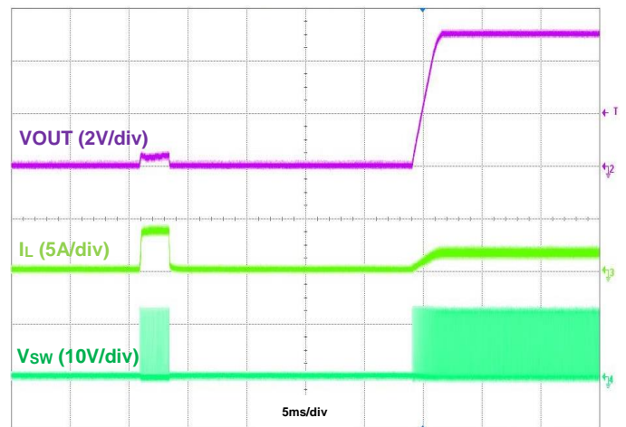
Figure 23. Output Short Recovery, IOU = 1.5A
