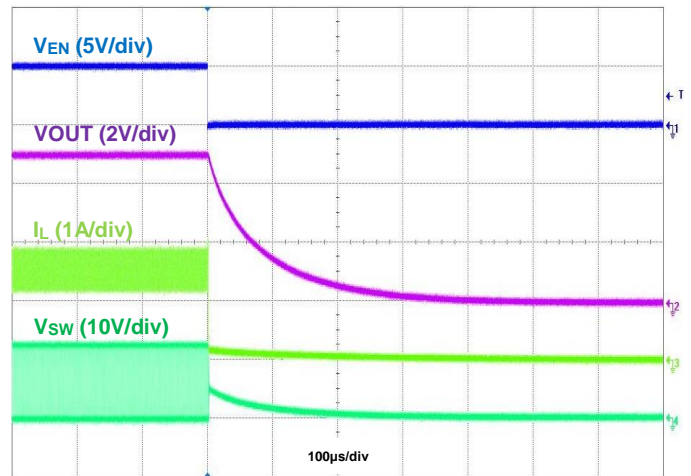
Figure 21. Shutdown Using EN, IOU = 1.5A
