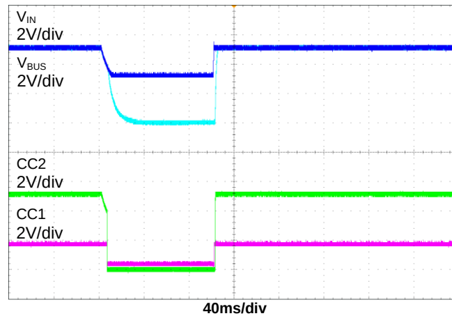
Figure 17. Brown-Out Test
