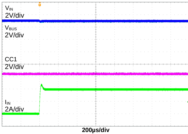
Figure 13. Load Step
