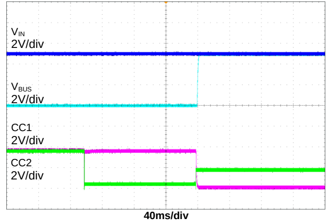
Figure 12. Start-Up
