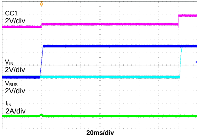
Figure 11. Basic Start-Up
