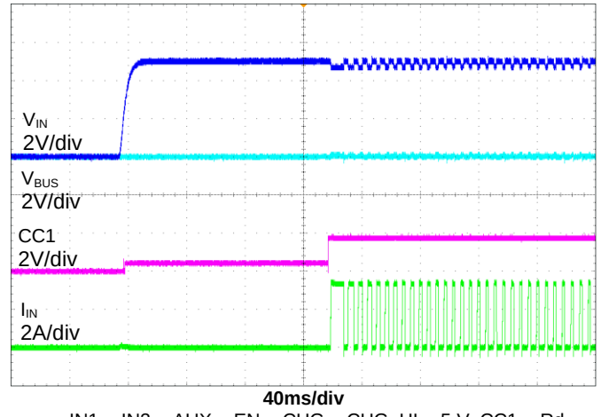
Figure 14. Hot-Plug to Short
