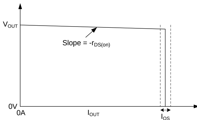
Figure 20 Current limit profile
