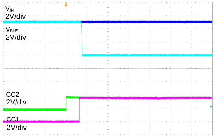
Figure 14. Hot-Plug to Short
