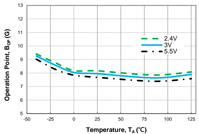
Operation Point BOP vs. Temperature
