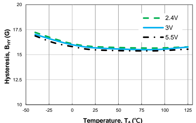
Hysteresis B_{HY} vs. Temperature
