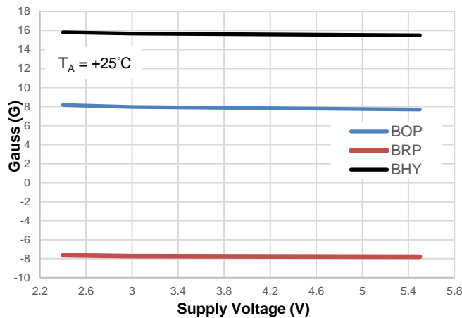
Switch Point vs. Supply Voltage V_{DD}
