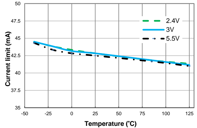
Current Limit I_{OCL} vs. Temperature
