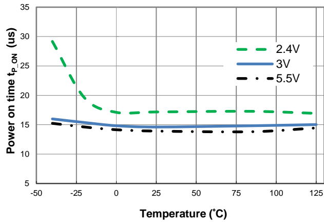
Power On Time t_{P\_ON} vs. Temperature
