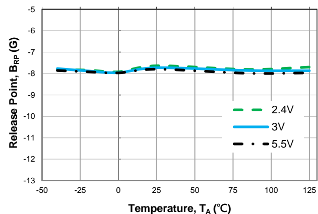
Release Point BRP vs. Temperature
