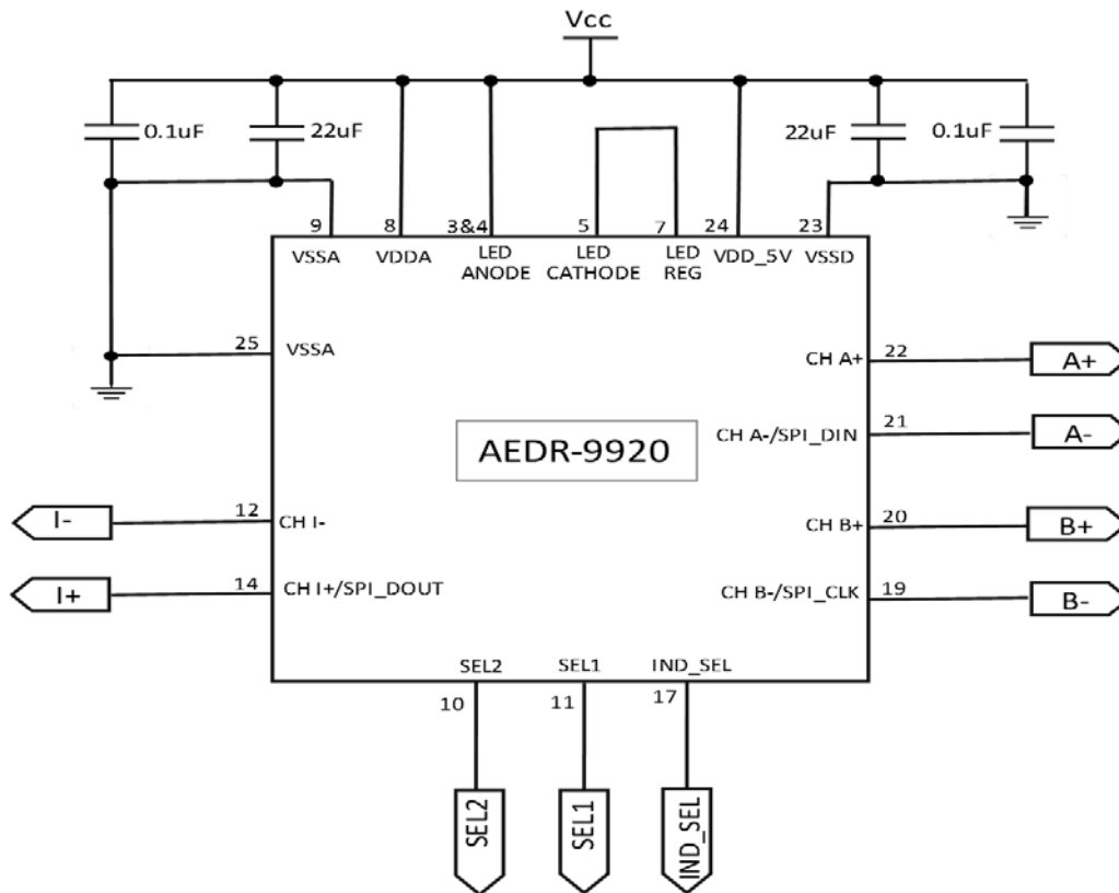
Figure 6: Power Supply Pins
