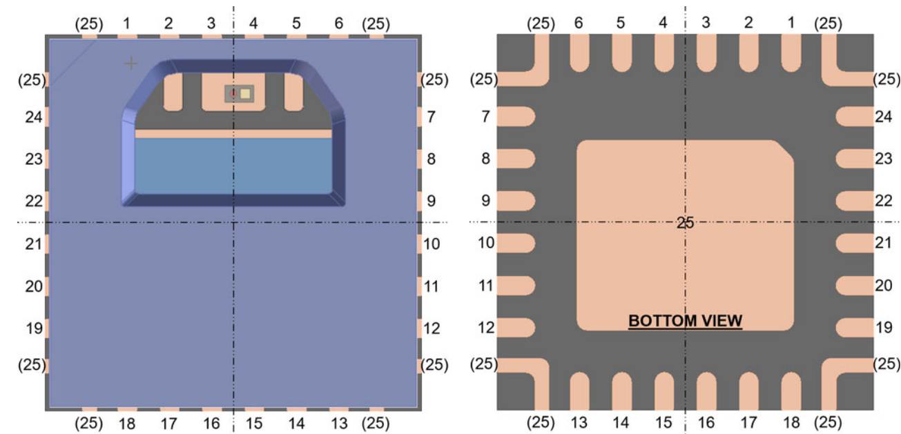
Figure 2: Encoder Pinout
