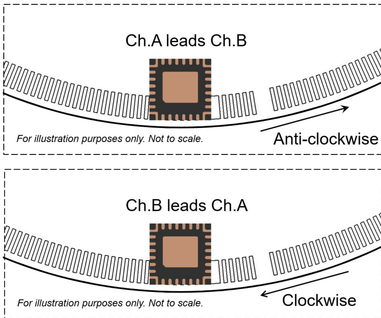
Figure 10: Channel A and Channel B
