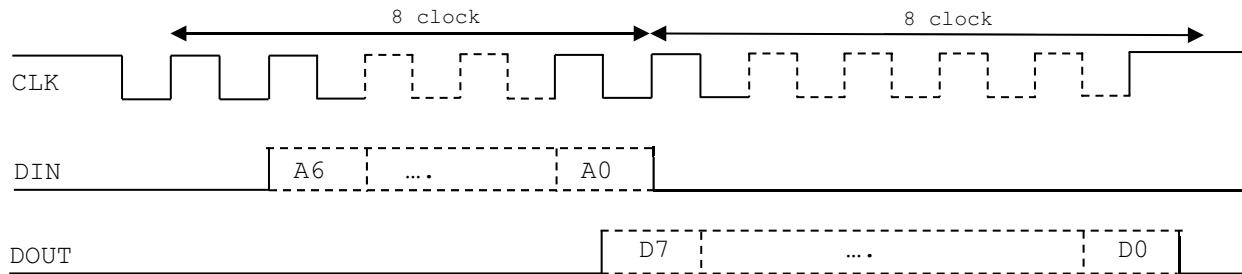
Figure 5: SPI Read Timing Diagram
