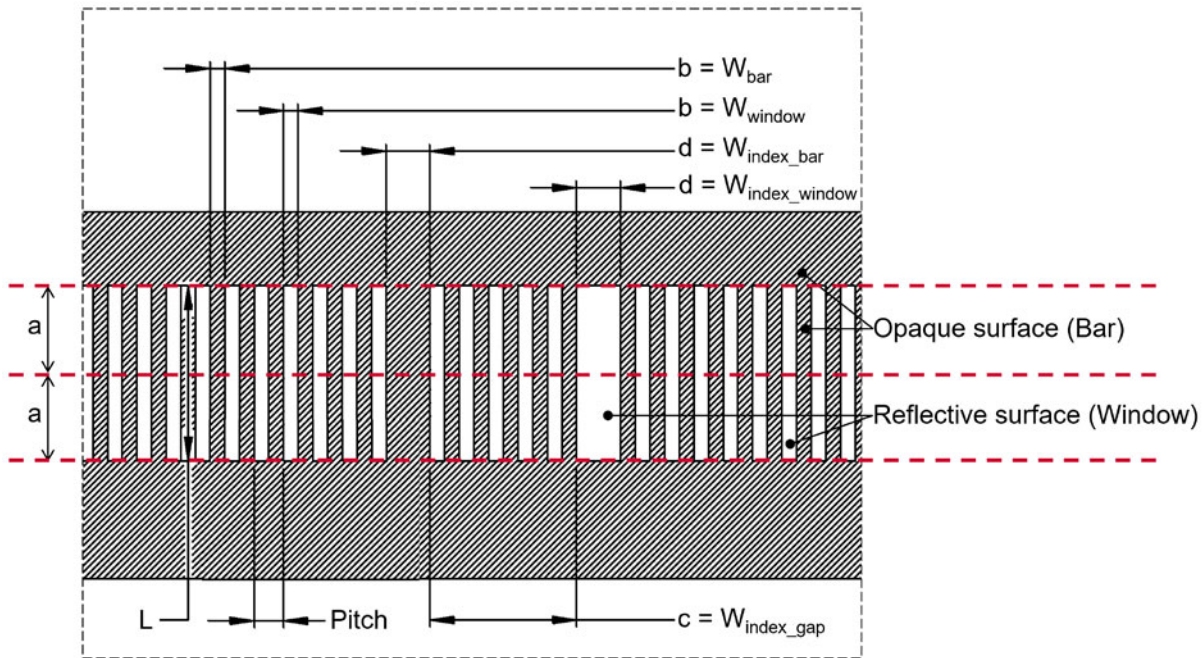
Figure 8: Code Strip Design
