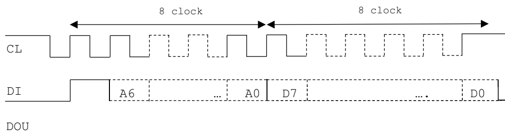
Figure 4: SPI Write Timing Diagram
