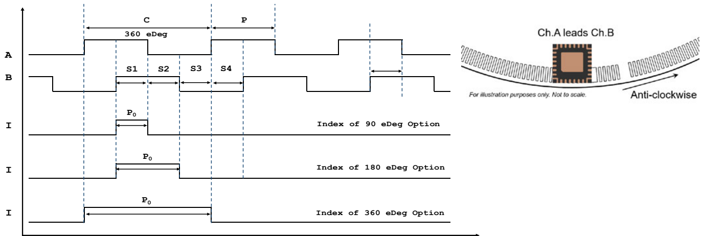
Figure 1: Output Waveform
