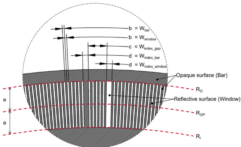
Figure 7: Code Wheel Design
