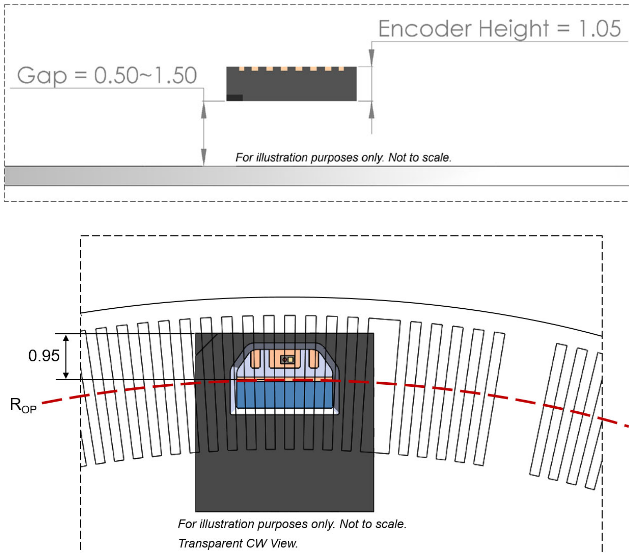
Figure 9: Encoder Placement
