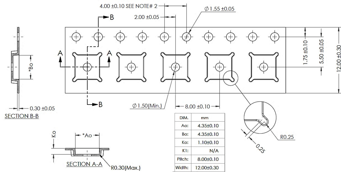
Figure 12: Tape and Reel
