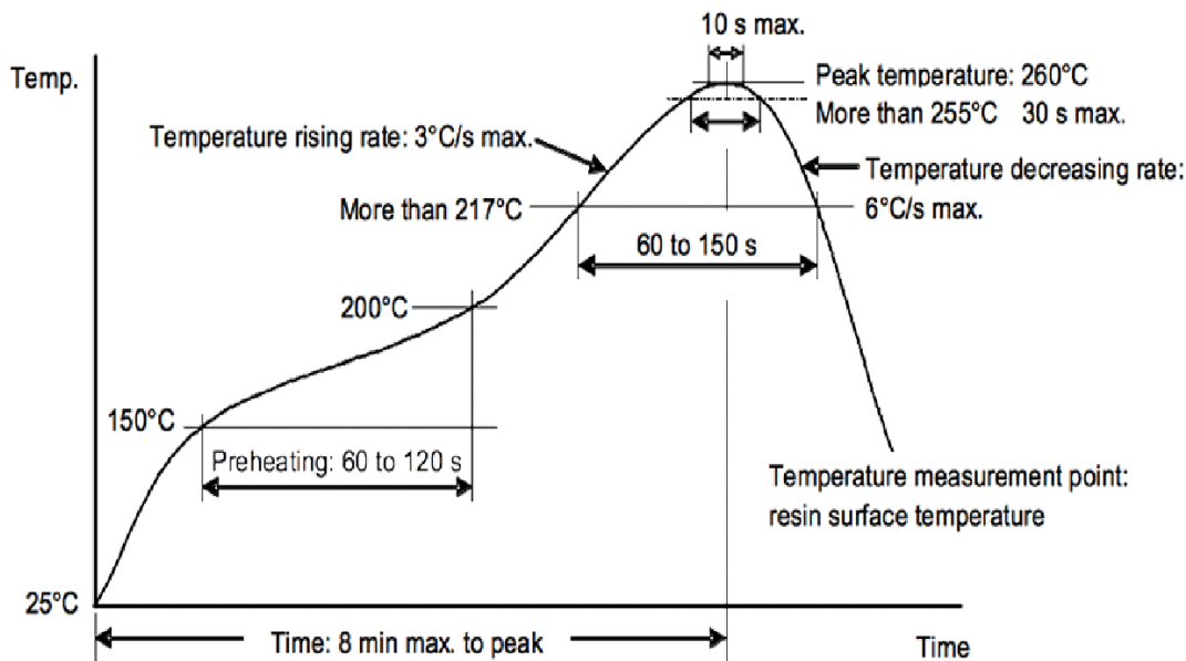
Figure 11: Recommended Lead-Free Solder Reflow Soldering Temperature Profile
