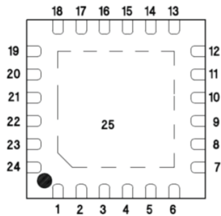
Figure 2 Pin Configurations
