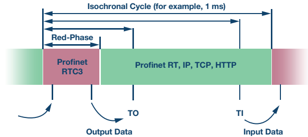
Figure 4. PROFINET IRT.
