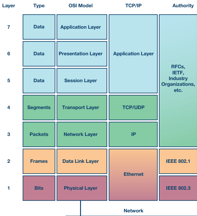
Figure 2. ISO seven-layer model.
