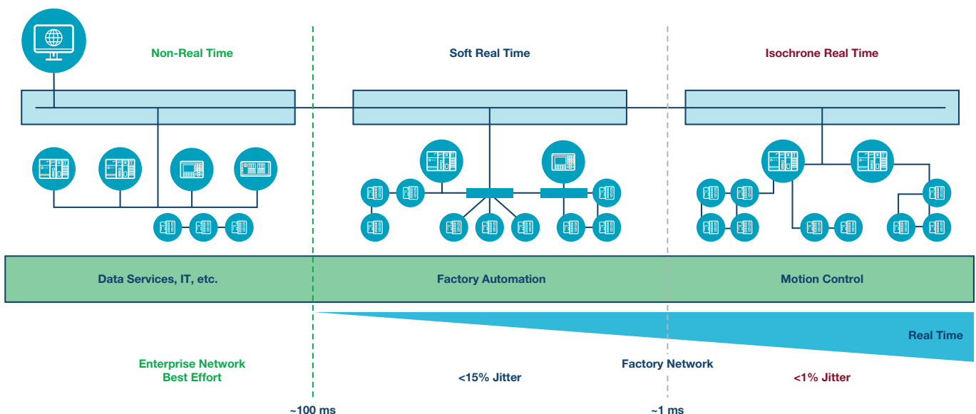
Figure 1. Real-time communications in automation.
