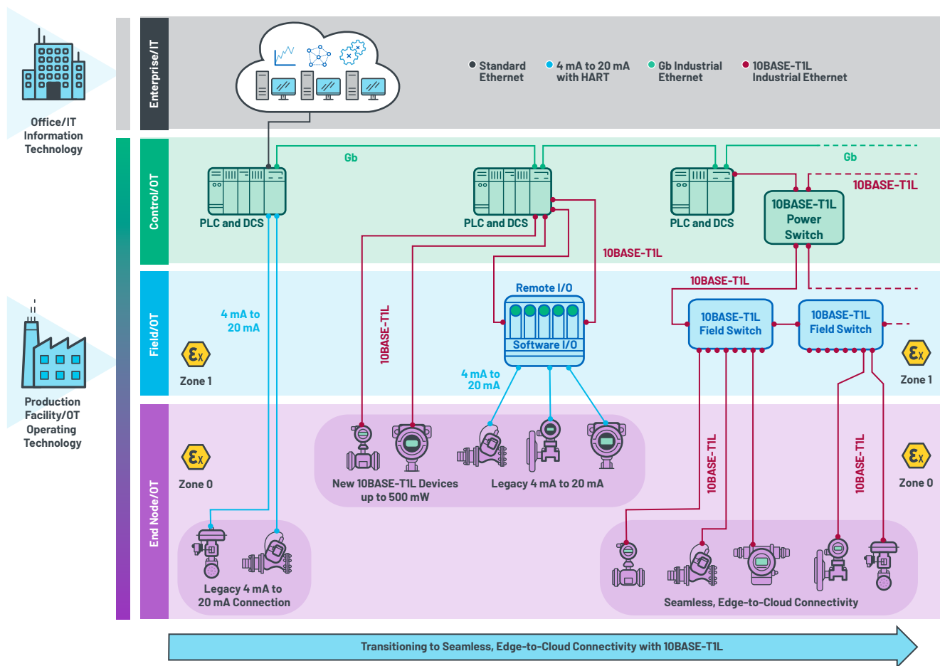
Figure 5. Legacy discrete wiring will gradually become a smart Ethernet network of all sensors and actuators.
