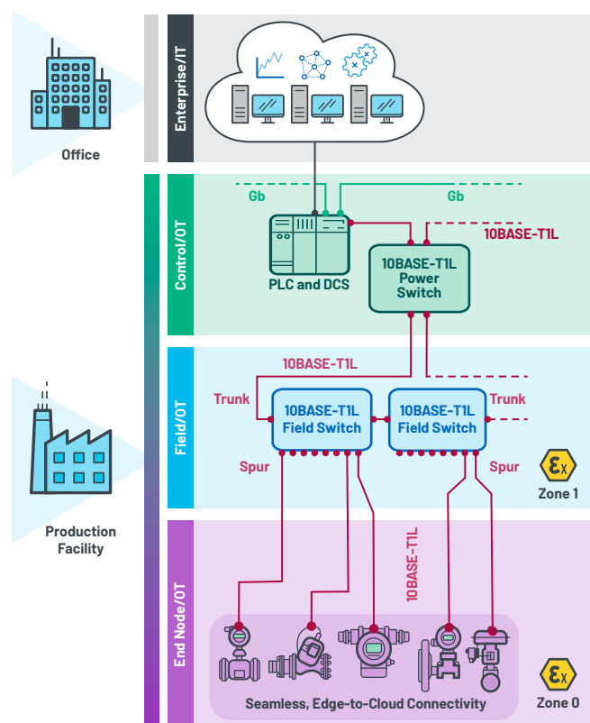
Figure 4. 10BASE-T1L network topology for the process industry.
