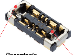
Receptacle, 211175 Series
