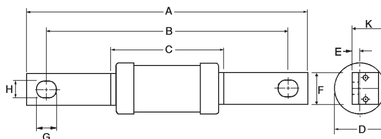
Dimensional Data
