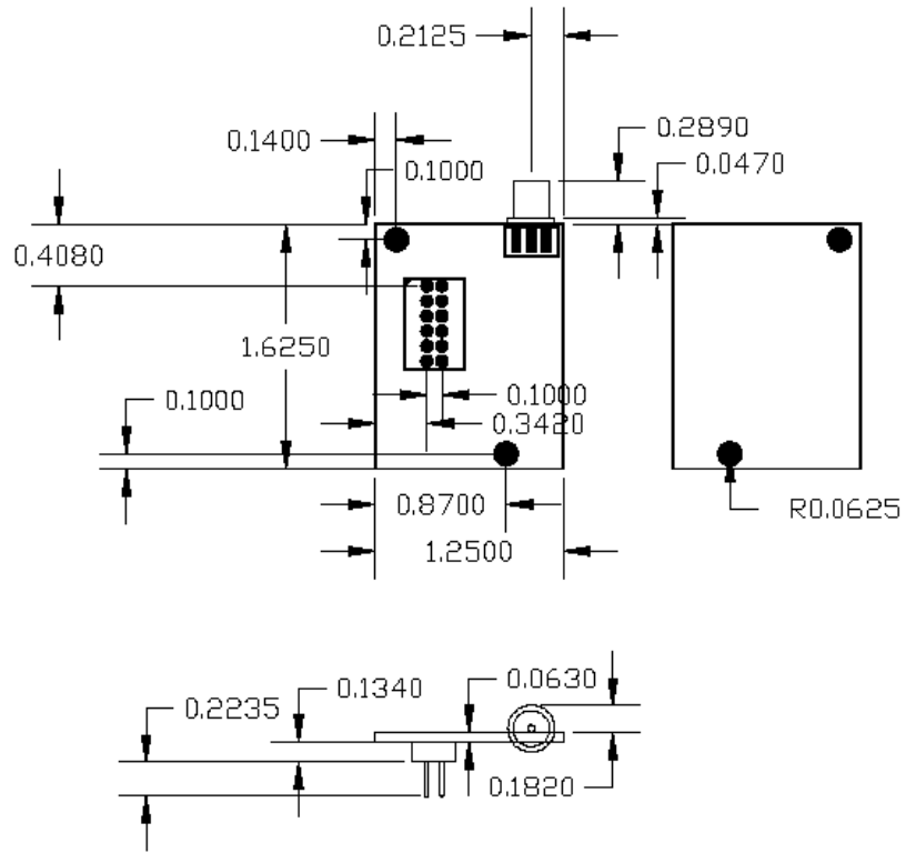
Figure 5-1: Mechanical Dimensions (all measures are in inches)
