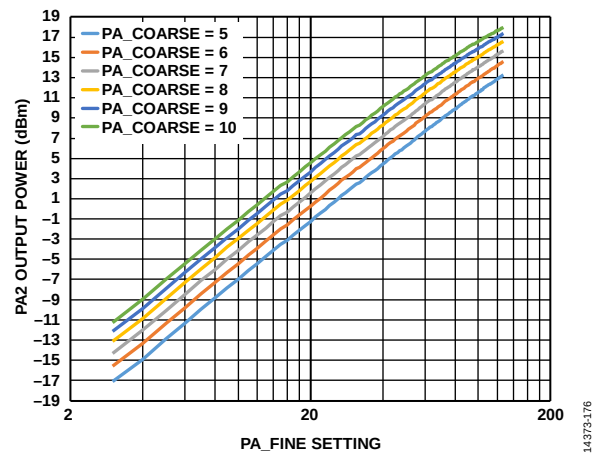
Figure 75. PA2 Output Power vs. PA_FINE Setting and PA_COARSE Setting with PA_FINE on a Logarithmic Scale, PAOLDO_VOUT_CON = 15, RF Frequency = 915 MHz, V_{DD} = 3.0 V, T_A = 25^\circ\text{C}
