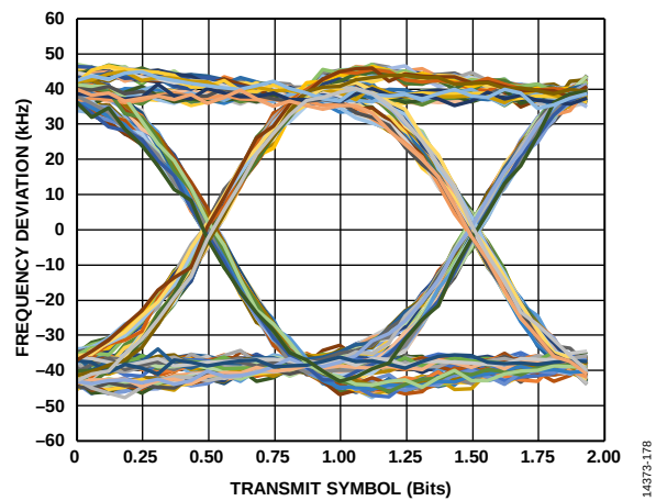
Figure 77. Transmit Eye Diagram, PA2 Output Power = 17 dBm, Configuration 915 MHz/150 kbps, V_{DD} = 3.0 V, T_A = 25^\circ\text{C}
