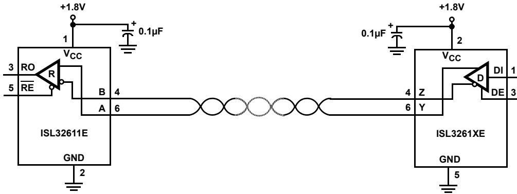
FIGURE 2. NETWORK WITH ENABLES
