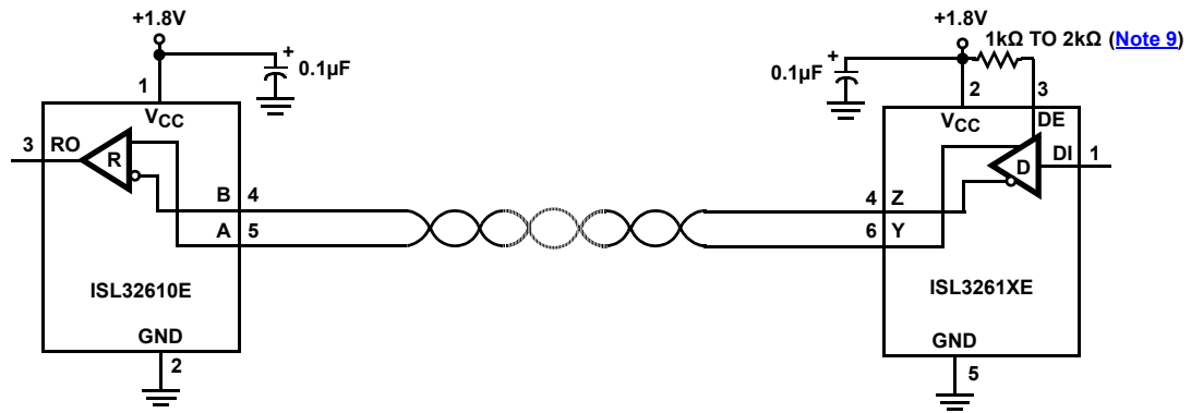
FIGURE 3. NETWORK WITHOUT ENABLES
