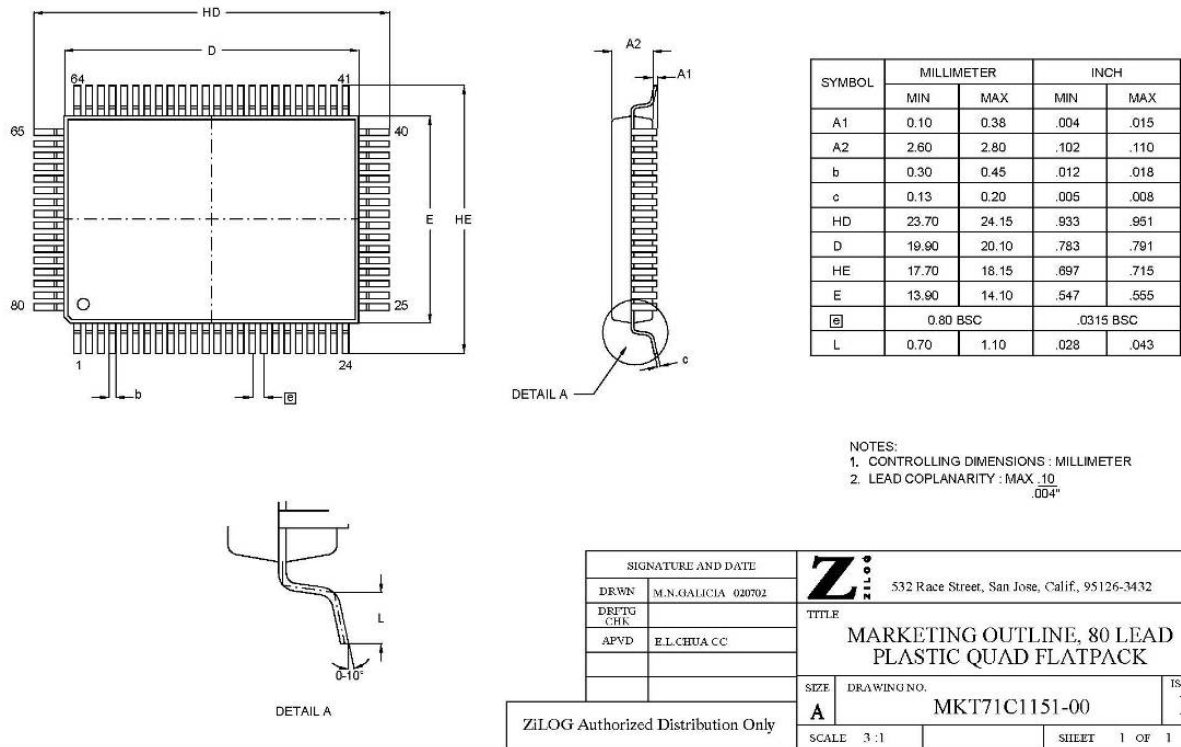
Figure 84. 80-Pin Quad-Flat Package (QFP)
