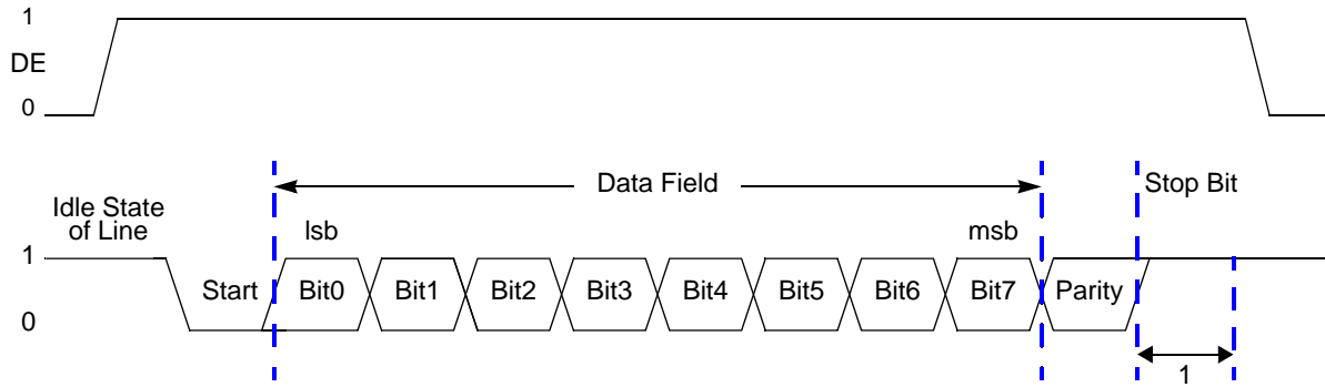
Figure 27. LIN-UART Driver Enable Signal Timing (shown with 1 Stop Bit and Parity)
