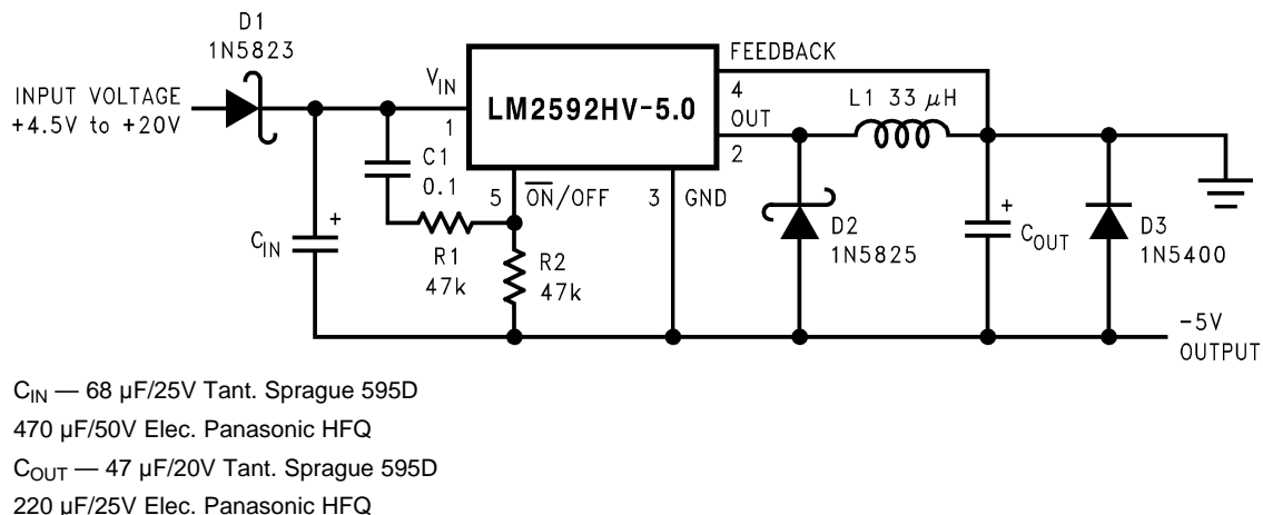
Figure 32. Inverting -5V Regulator with Delayed Startup
