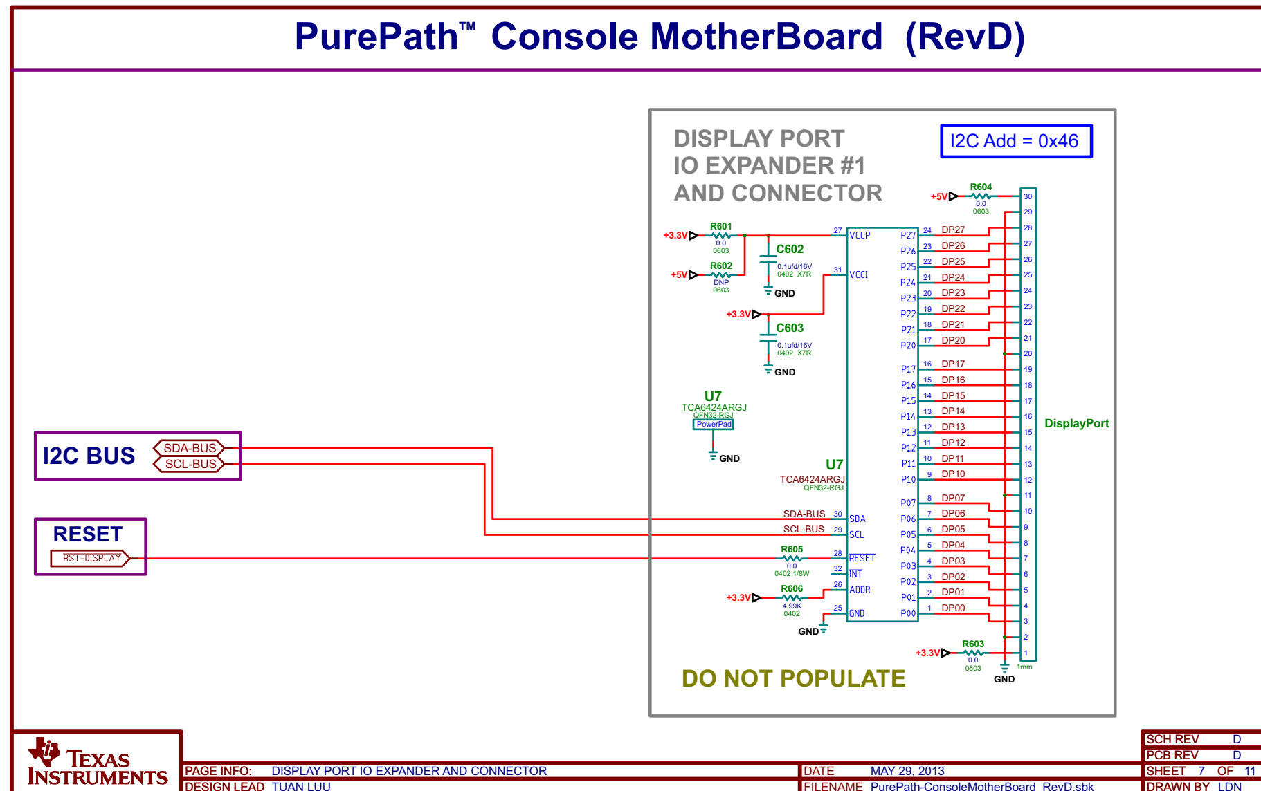
Figure 27. PurePath Console Revisions D and E (7 of 10)
