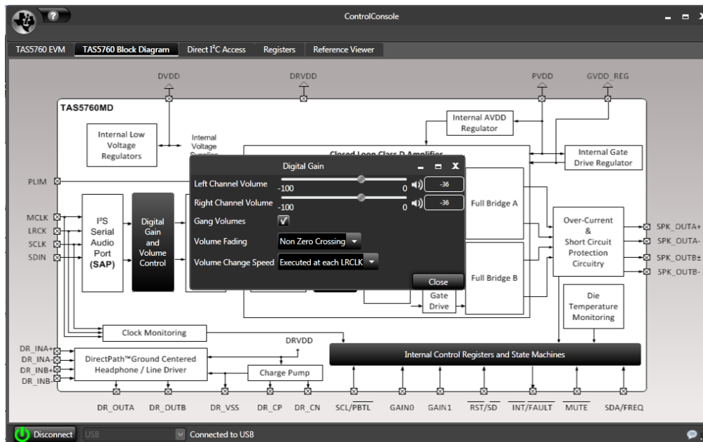
Figure 9. Digital Gain Pop-Up
