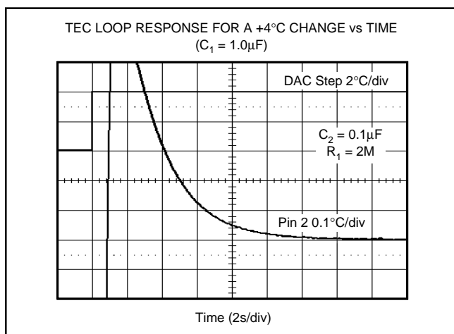
FIGURE 11. TEC Loop Response for a +4°C Change vs Time ( C_1 = 1.0\mu\text{F} ).
