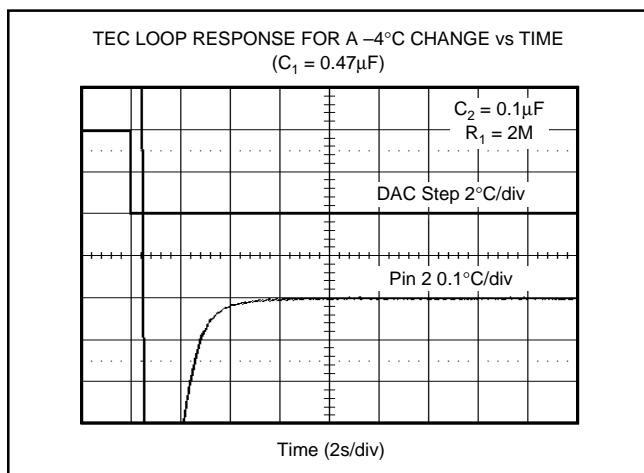
FIGURE 10. TEC Loop Response for a -4°C Change vs Time ( C_1 = 0.47\mu\text{F} ).
