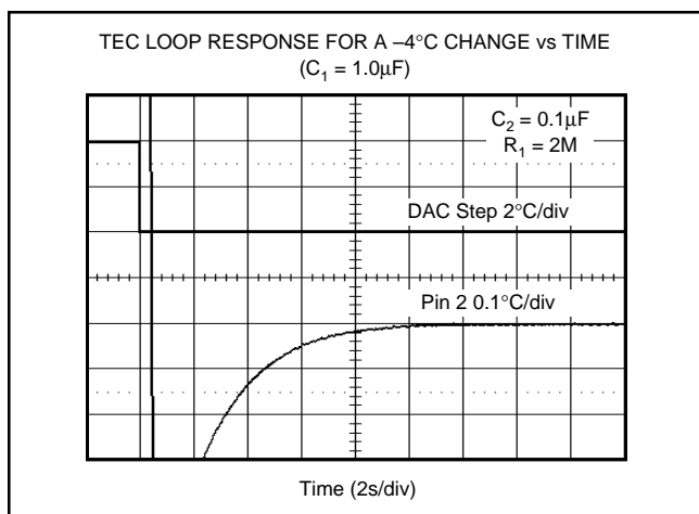
FIGURE 9. TEC Loop Response for a -4°C Change vs Time ( C_1 = 1.0\mu\text{F} ).
