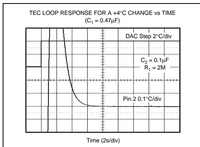
FIGURE 12. TEC Loop Response for a +4°C Change vs Time ( C_1 = 0.47\mu\text{F} ).
