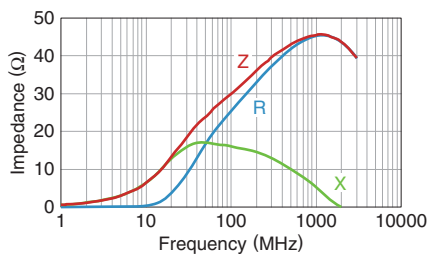
MPZ1005Y900C
