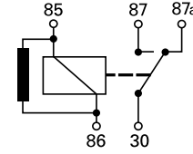
Change Over with resistor (B)
