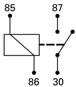
Normally open (A)
