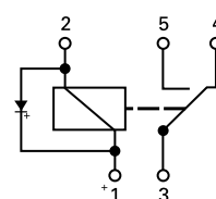
Change Over with Diode (C)
