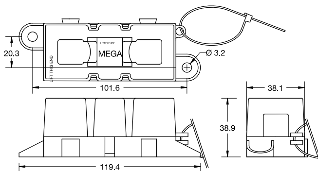
Dimensions in mm / Maße in mm
