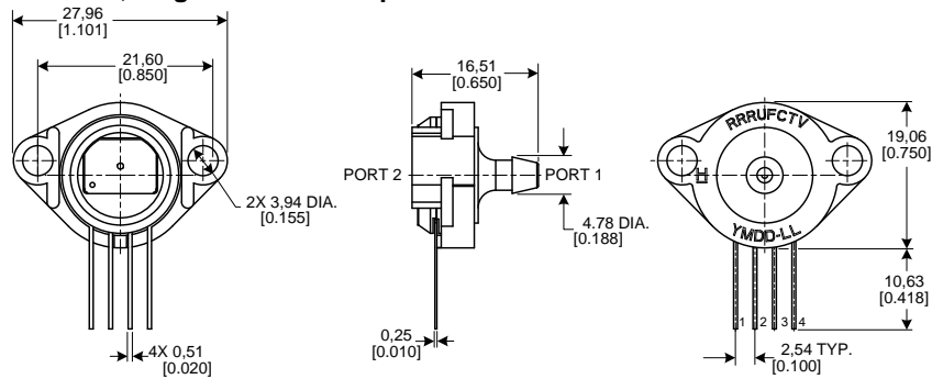
Figure 8. SIP Package Dimensional Drawings (continued)
