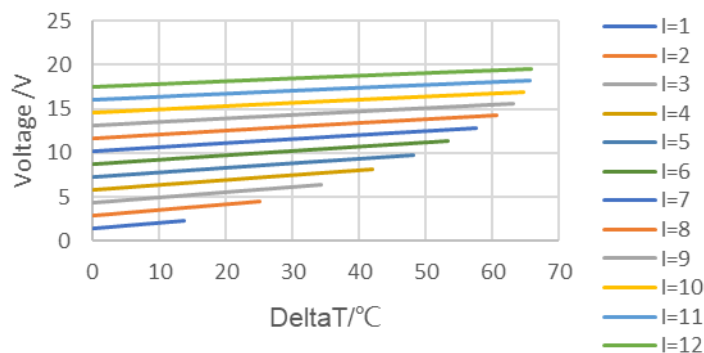
Performance Curves at T_h = 27^\circ\text{C}
