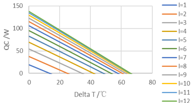
Performance Curves at T_h = 27^\circ\text{C}
