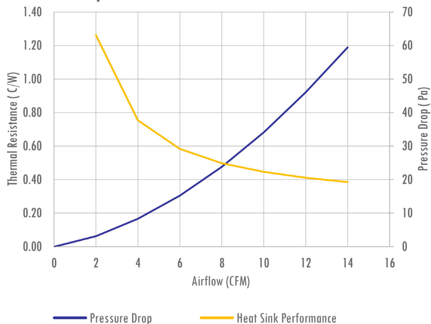
System Curve for ATS-KRA-3559-C1-R0
