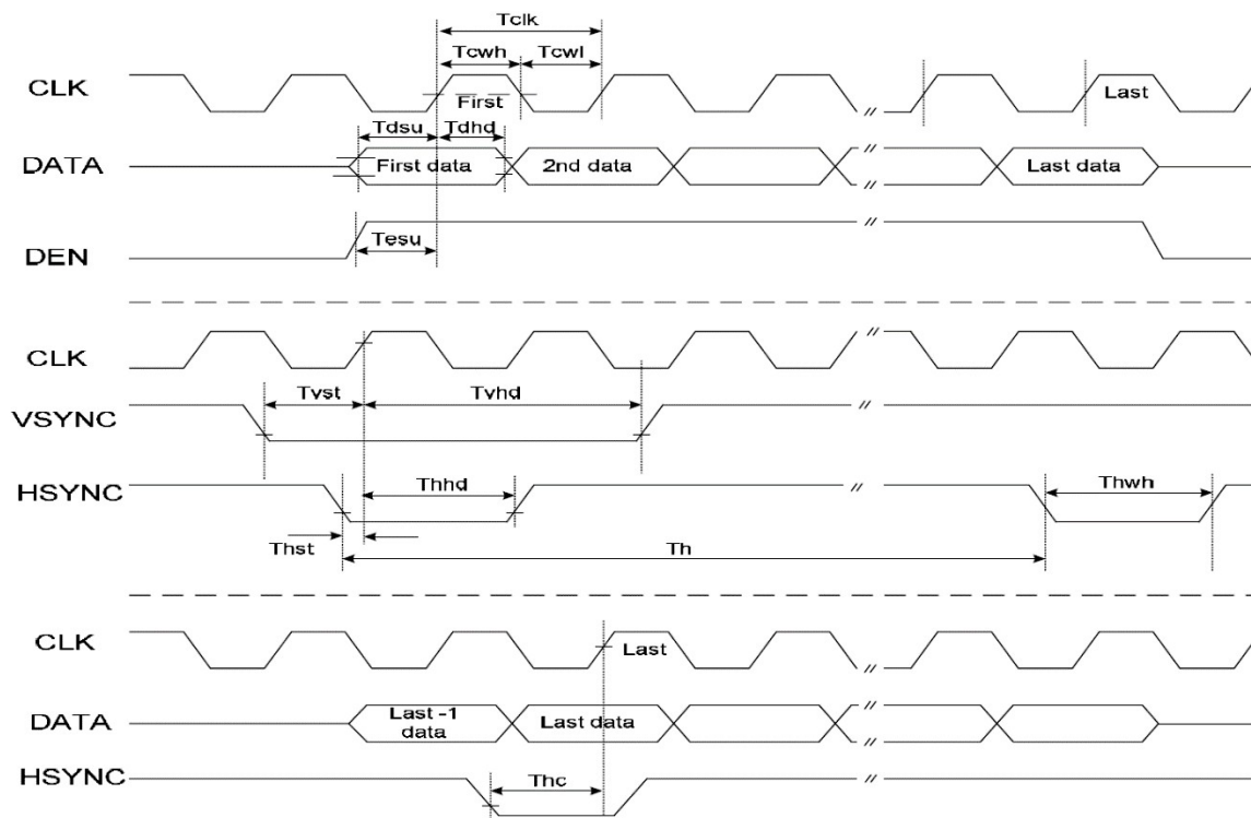
LCD Timing Chart
