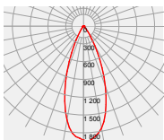
CREE CXA1520
