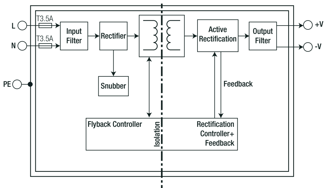
Blockdiagram (“/ENC/2x4”)
