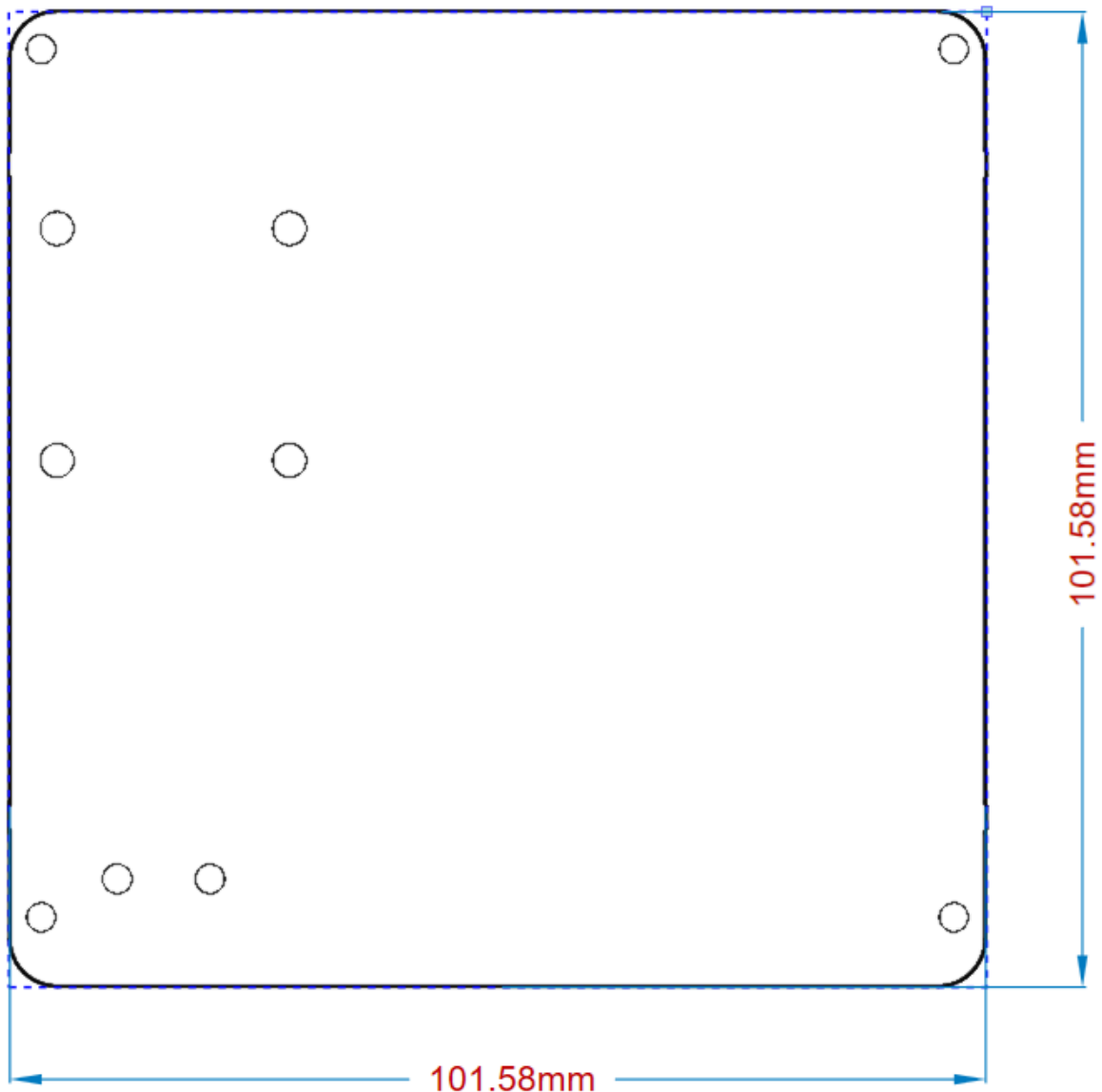
Board outline
