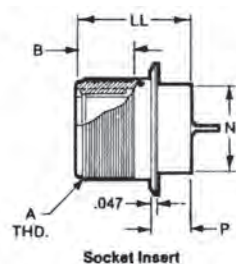
Socket Insert
