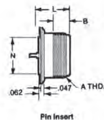
Pin Insert
