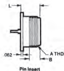
Pin Insert
