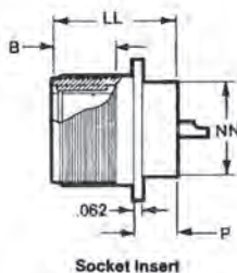
Socket Insert
