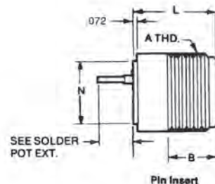
Pin Insert
