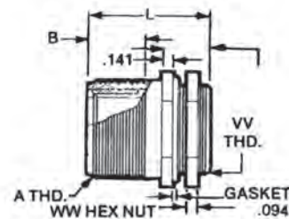
Socket Insert
