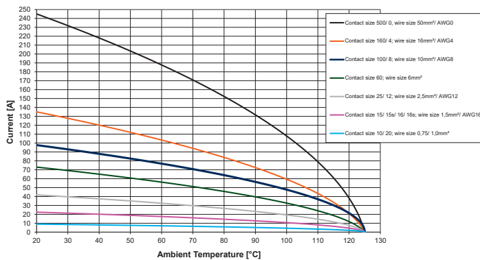
Derating Curves according to VG 95342
