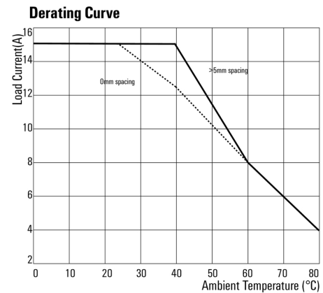
Derating curve
