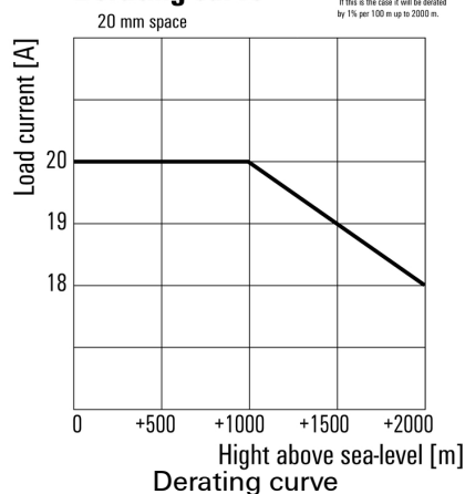
Derating curve
