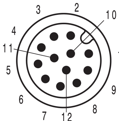
Pole scheme
