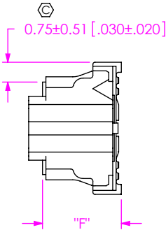
FIG 3 -K: KAPTON OPTION SS5-20-3.00-X-D-K-XR SHOWN (USE K-DOT-.138-.250-.005) (DIFFERENT AS SHOWN, OTHERWISE SAME AS FIG 1)
