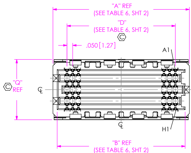
FIG 2 -06.5 THRU -13.0 LEAD STYLES (SEAM-20-09.0-XXX-08-1-A-XR SHOWN) (SAME AS FIG 1, EXCEPT AS SHOWN) (SOME CENTER FEATURES REMOVED FOR CLARITY)
