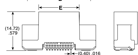
P1M-10-01-S-DV SHOWN
