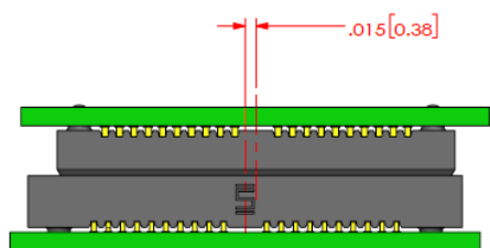
INITIAL X AXIS LINEAR MISALIGNMENT
