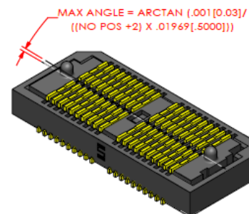
INITIAL Z AXIS ANGULAR MISALIGNMENT
