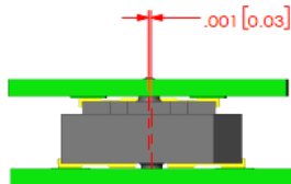
FINAL Y AXIS LINEAR MISALIGNMENT
