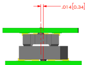
INITIAL Y AXIS LINEAR MISALIGNMENT
