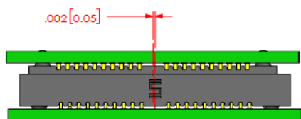
FINAL X AXIS LINEAR MISALIGNMENT
