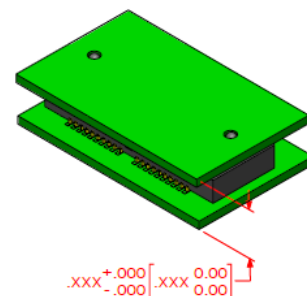
INITIAL Z AXIS LINEAR MISALIGNMENT
