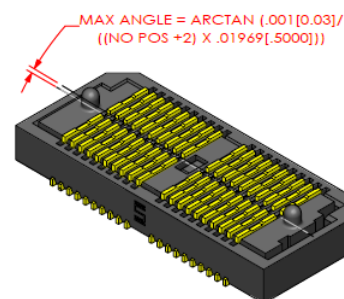
FINAL Z AXIS ANGULAR MISALIGNMENT
