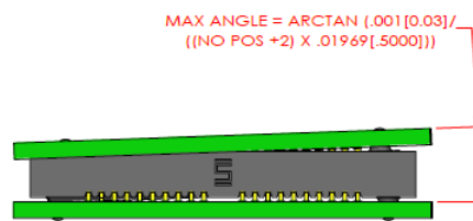
FINAL Y AXIS ANGULAR MISALIGNMENT
