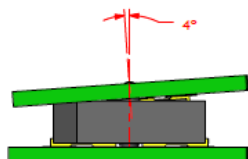
INITIAL X AXIS ANGULAR MISALIGNMENT
