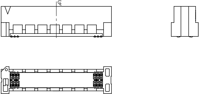
FIG 6 HTEC8-130-01-X-DV SHOWN (DIFFERENT AS SHOWN, OTHERWISE SAME AS FIG 1) (SOME FEATURES NOT SHOWN FOR CLARITY)
