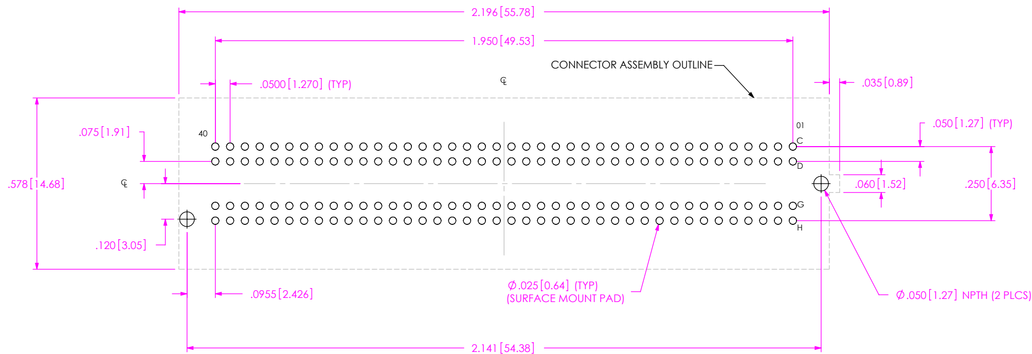
RECOMMENDED PCB LAYOUT ALL DIMENSIONS ARE SYMMETRICAL ABOUT CENTERLINE
