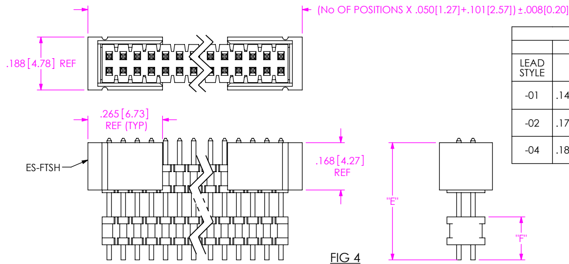
FIG 4 -ES OPTION FW-50-02-XX-D-610-075-ES (DIFFERENT AS SHOWN, OTHERWISE AS FIG 1) (BOARD SPACE .215-.610[5.46-15.49])
