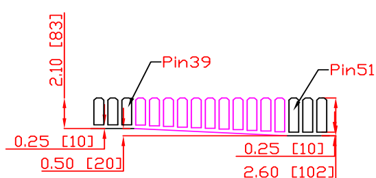
Detail C 30μ inch gold finger
