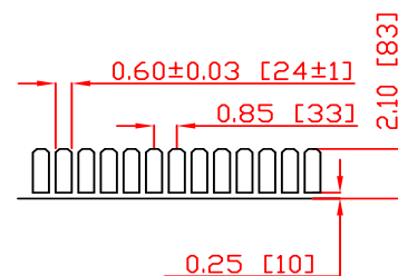
Detail B
