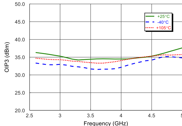
Channel B OIP3 over swept Frequency (& Temp.) with P_{OUT}/\text{Tone} = 3 dBm & 10 MHz tone spacing in HGM.
