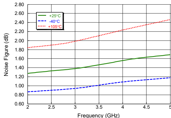
Channel B LNA Noise Figure over swept Frequency (& Temp.) in Rx High Gain Mode
