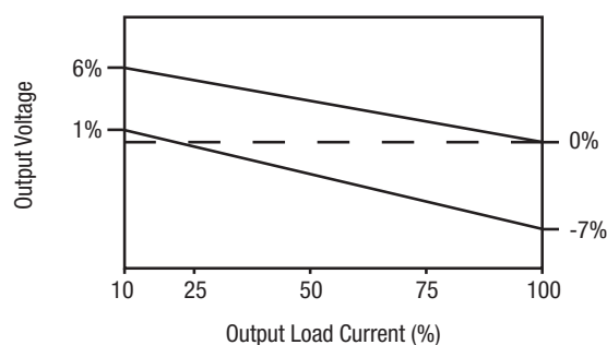
MEJ2S0503SC
