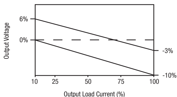
MEJ2S0503SC
