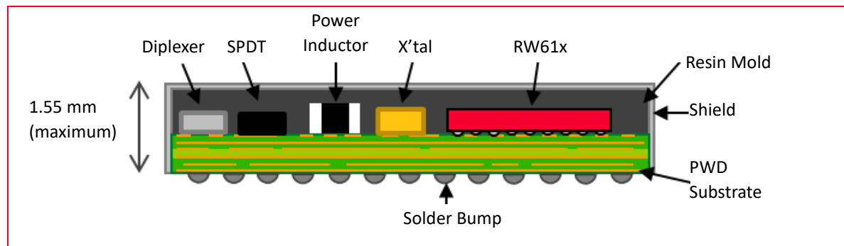
Figure 3: Structure
