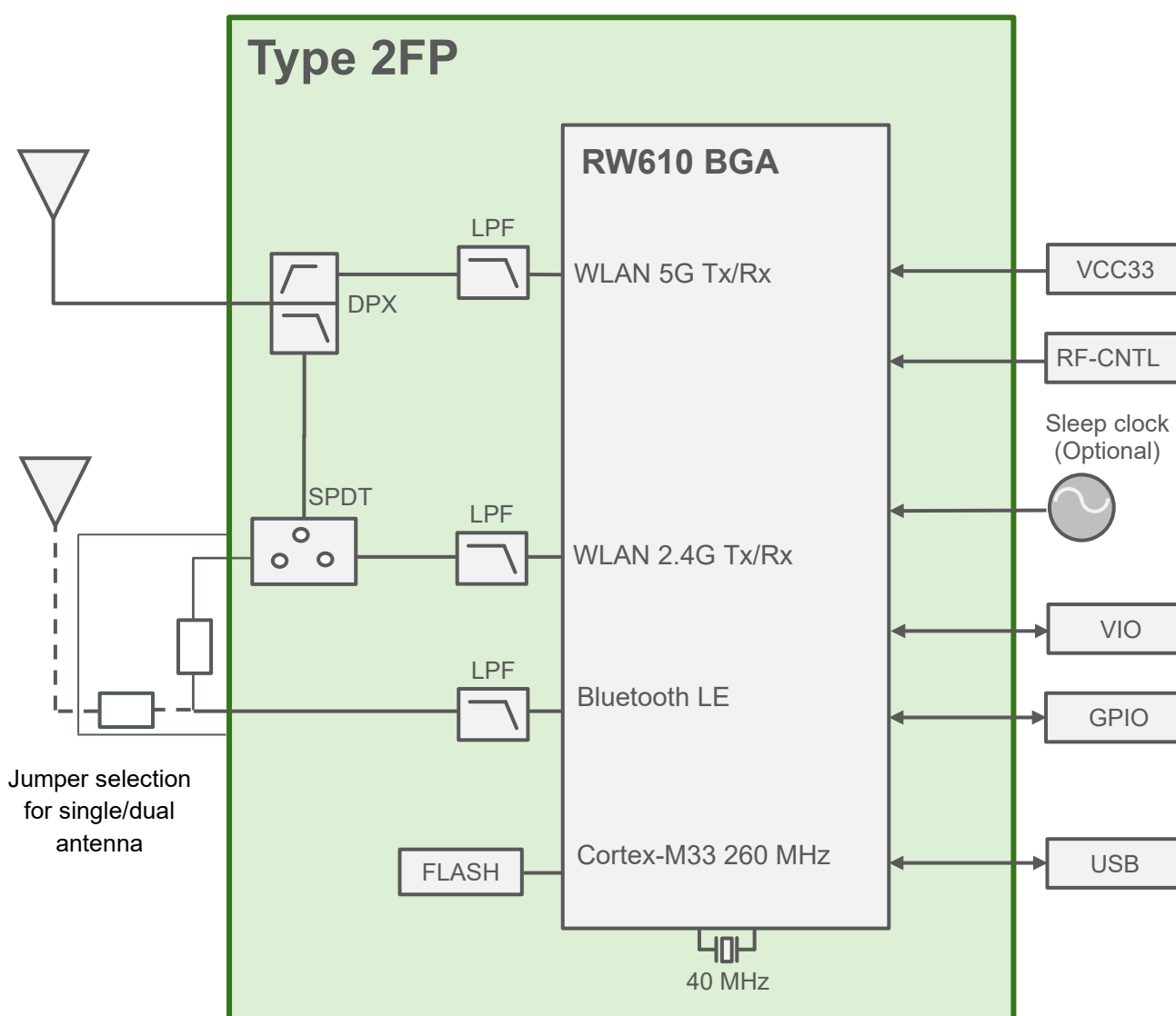
Figure 1: Block Diagram
