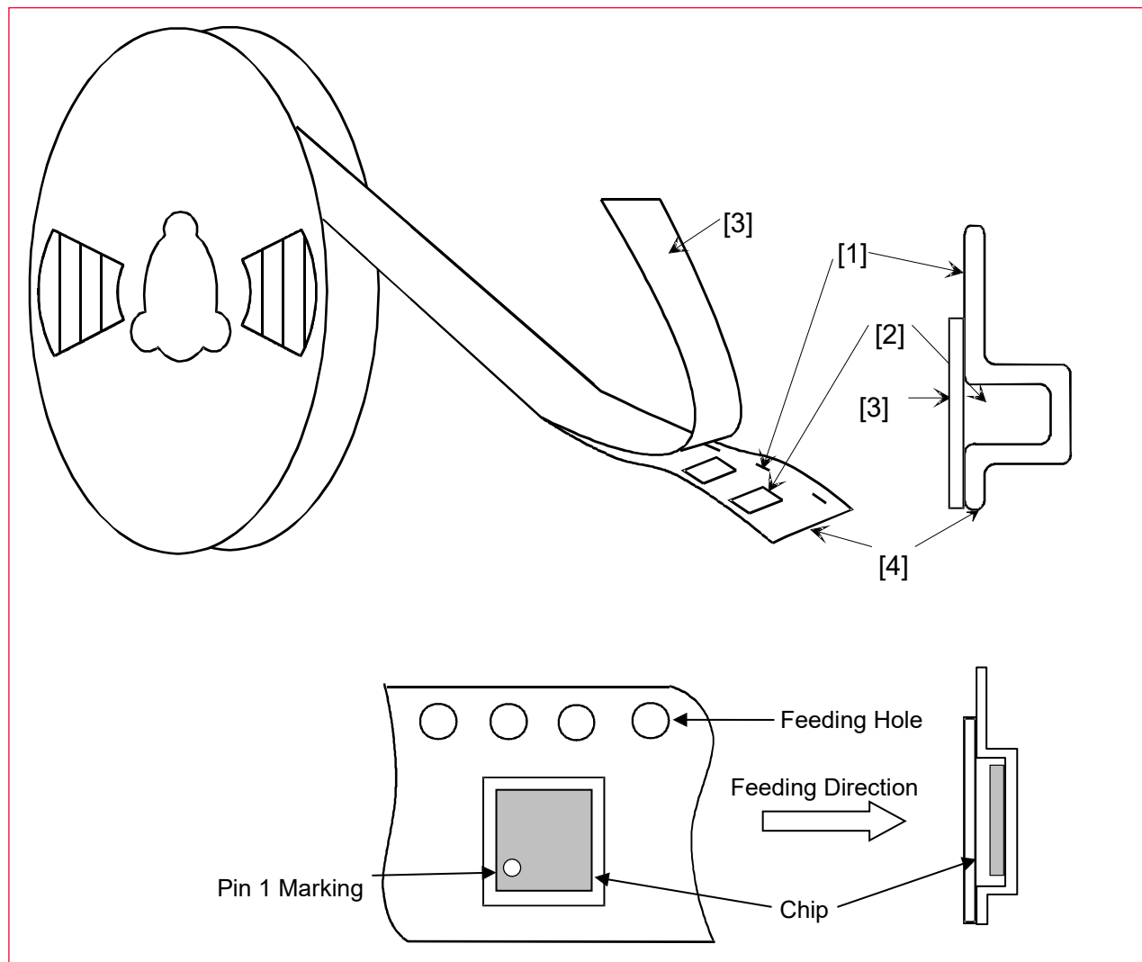
Figure 7: Taping Diagrams
