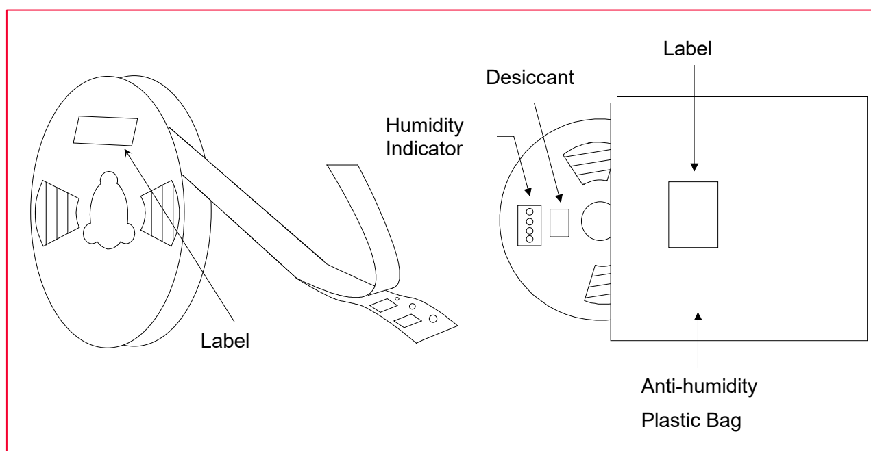
Figure 10: Humidity Proof Packing
