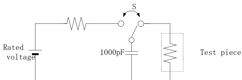
Fig 1 Pulse test circuit
