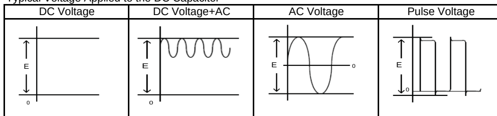
Typical Voltage Applied to the DC Capacitor
