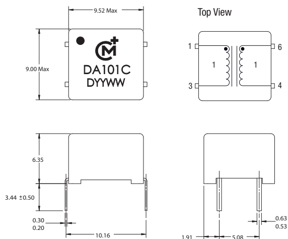
6 Pin DIL
