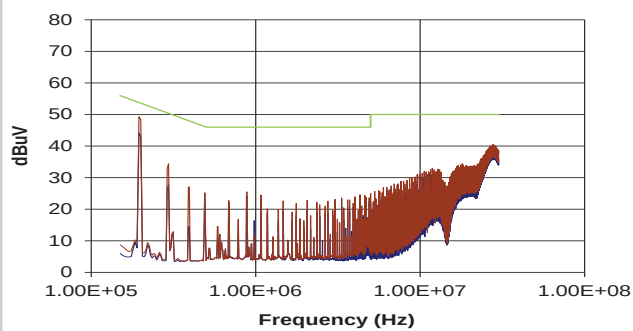
MGJ6D24H24MC (Average)
