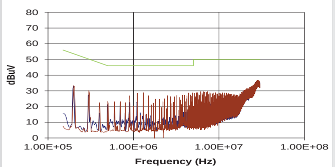
MGJ6D12H24MC (Average)
