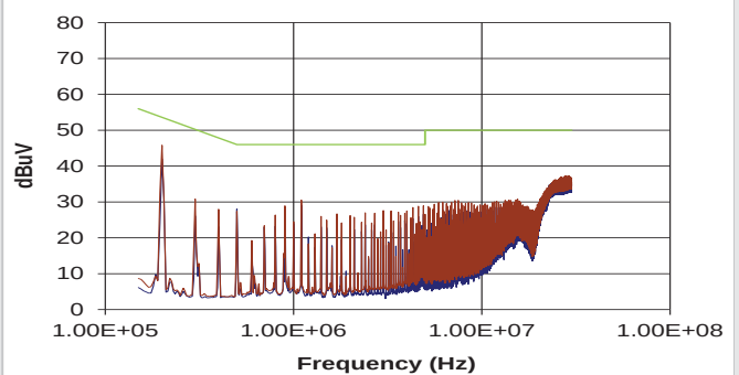
MGJ6D12H24MC (Average)
